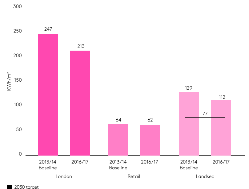
Landsec energy intensity Table 102
